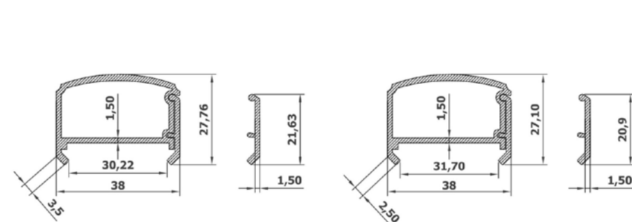
Continuous horizontal profile / Perfil horizontal continuo
