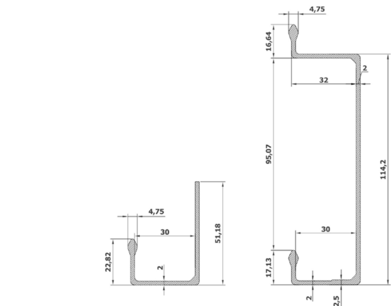
Profile single and double continuous / Perfiles continuos doble-simple
